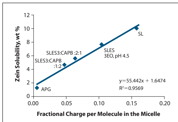
Figure 1. Correlation with micellar diffuse layer charge. Surfactant at 5% > 10 critical micellar charge in all cases. APG indicates alkyl polyglucoside; SLES:CAPB, sodium laureth sulfate:cocamidopropyl betaine; SLS, sodium lauryl sulfate; SL, sodium laurate.
